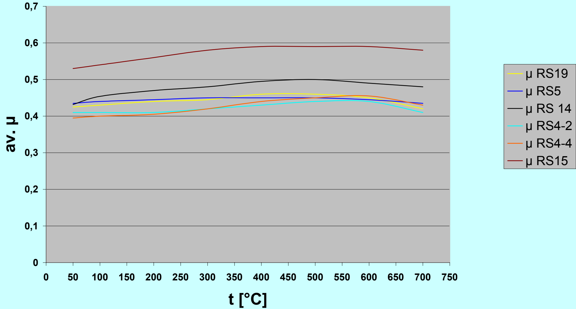
PAGID RS friction vs. temp
